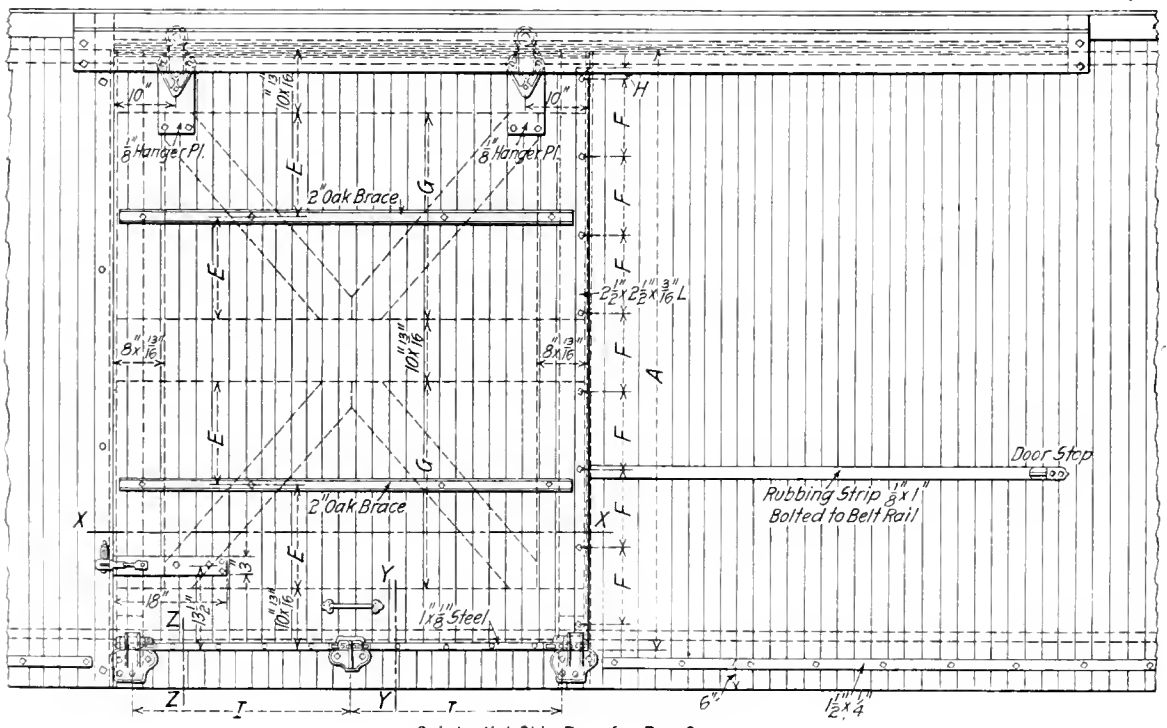
Substantial Side Door for Box Cars
